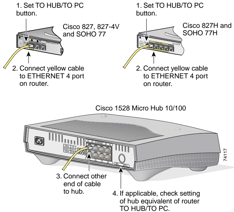
Figure 2-4 Connecting a Hub to the Router
