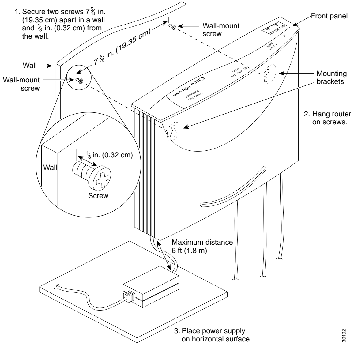
Figure 2-3 Mounting Router on a Wall
