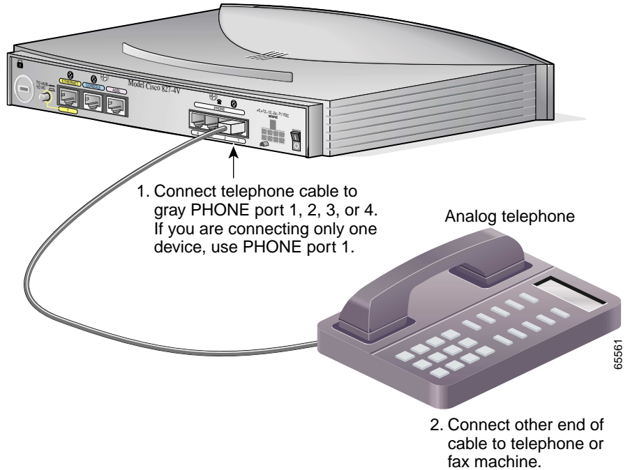
Figure 2-7 Connecting an Analog Telephone or Fax Machine
