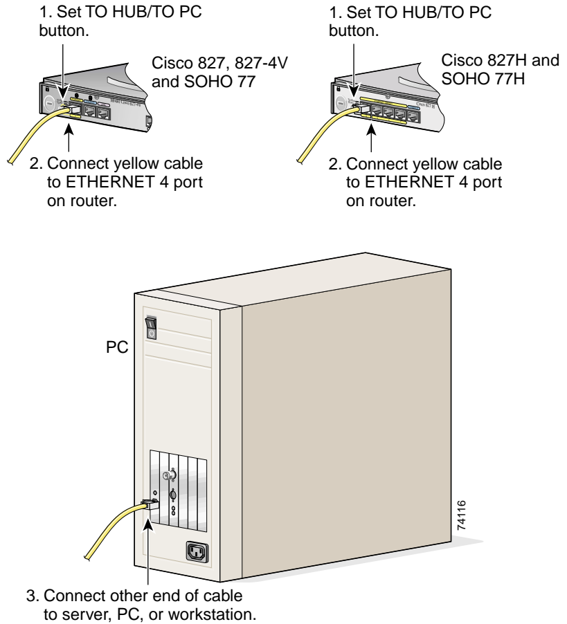
Figure 2-5 Connecting a Server, PC, or Workstation to the Router
