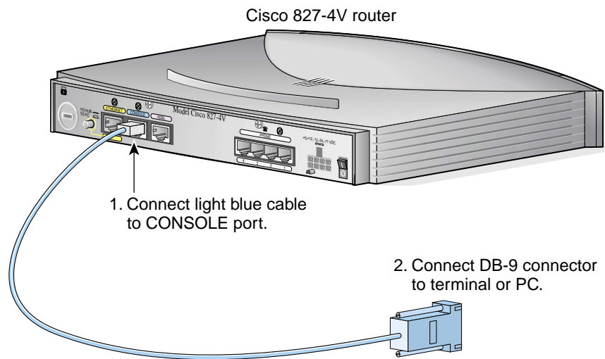
Figure 2-8 Connecting a Terminal or PC
