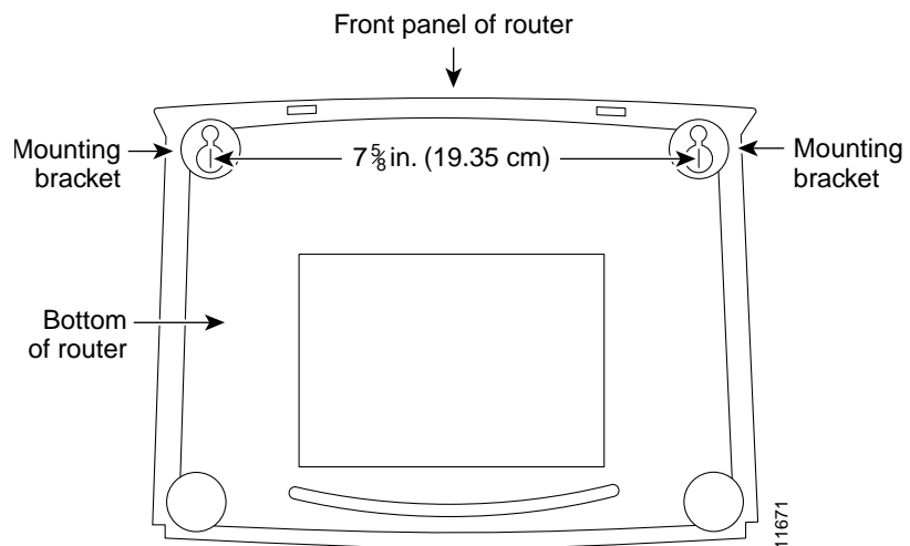
Figure 2-2 Wall-Mounting Brackets (Bottom of Router)
