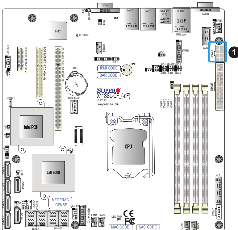
1. 8-Pin PWR
