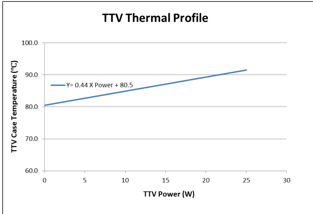
Figure 5-3. Thermal Test Vehicle Thermal Profile for Quad Core GT2 25W Processor
