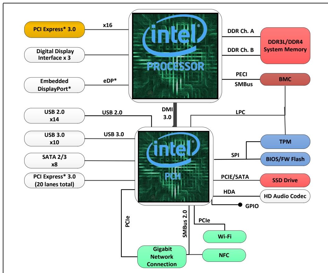
Figure 1-1. Platform Block Diagram
