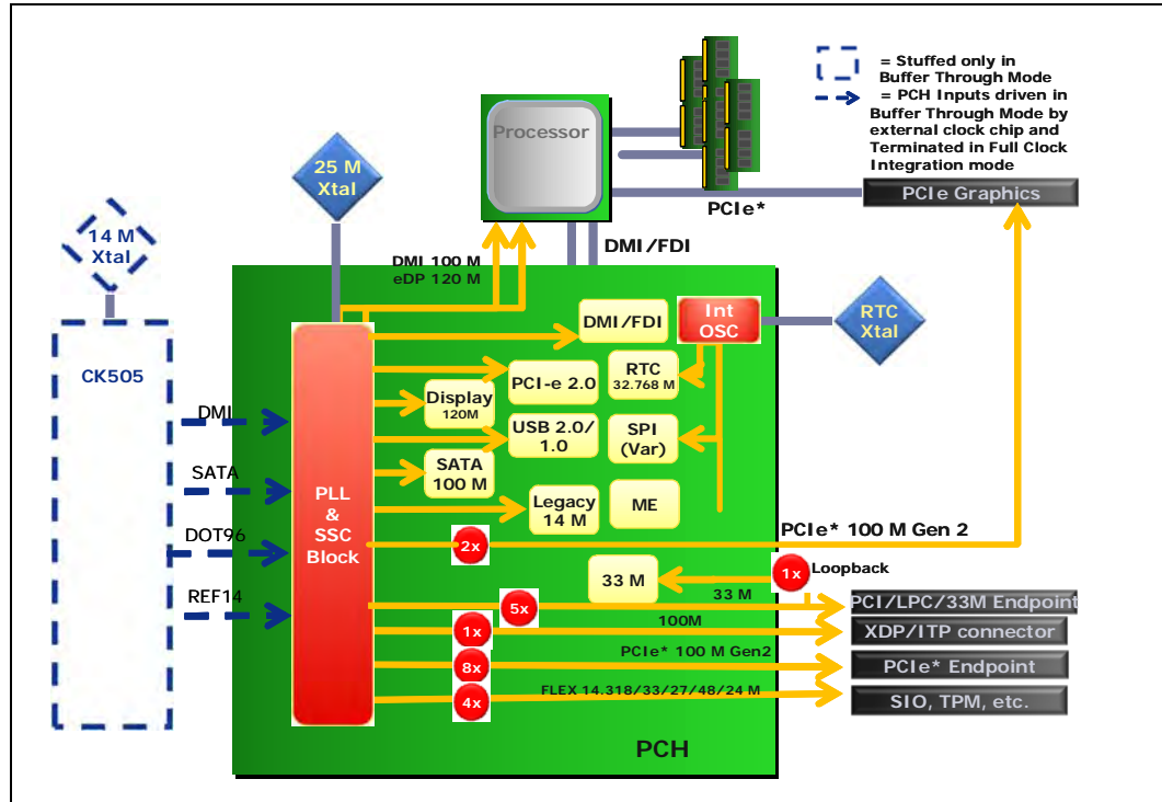
Figure 4-1. PCH High-Level Clock Diagram (Integrated Clock Mode)
