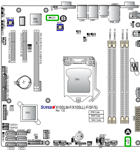
A. Onboard PWR LED
