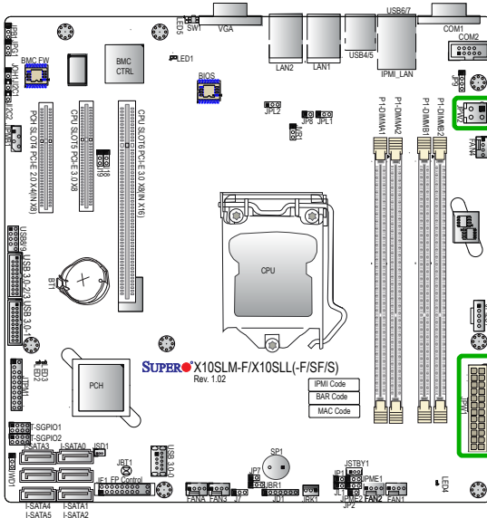
24-Pin Main PWR (Required)
