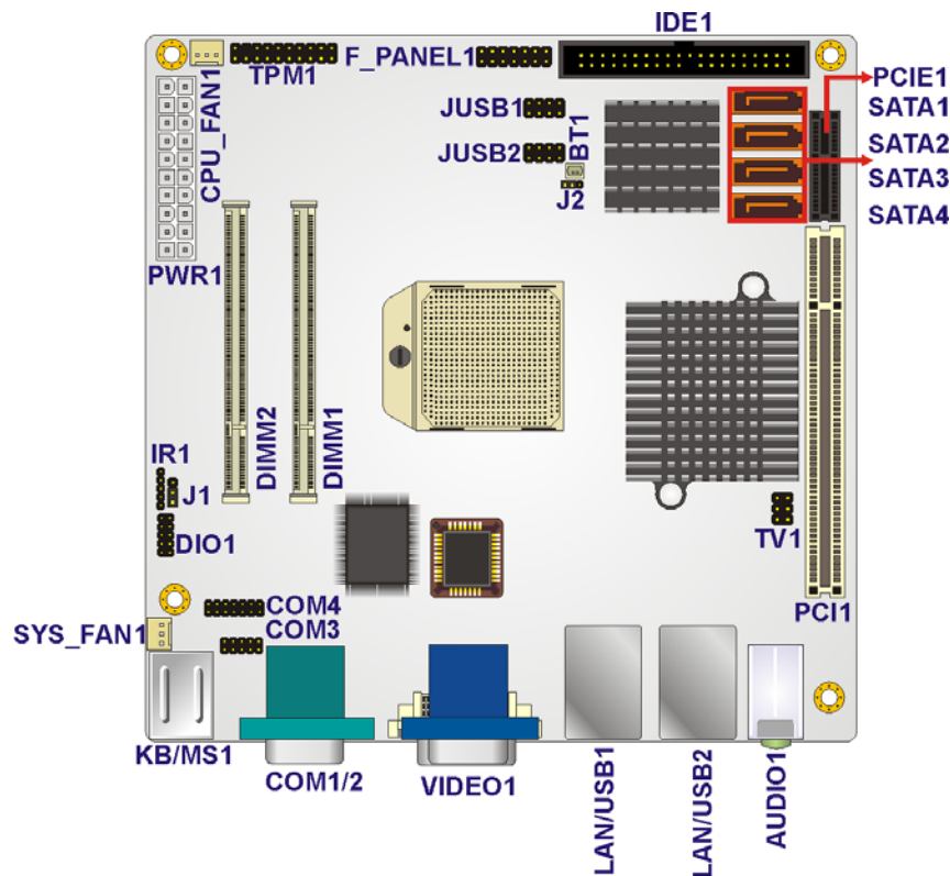
Figure 4-1: Connector and Jumper Locations
