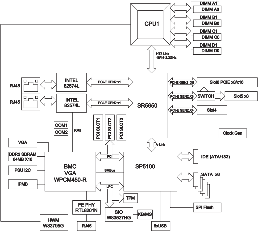
Figure 1-3. AMD SR5650/SP5100 Chipset: System Block Diagram
