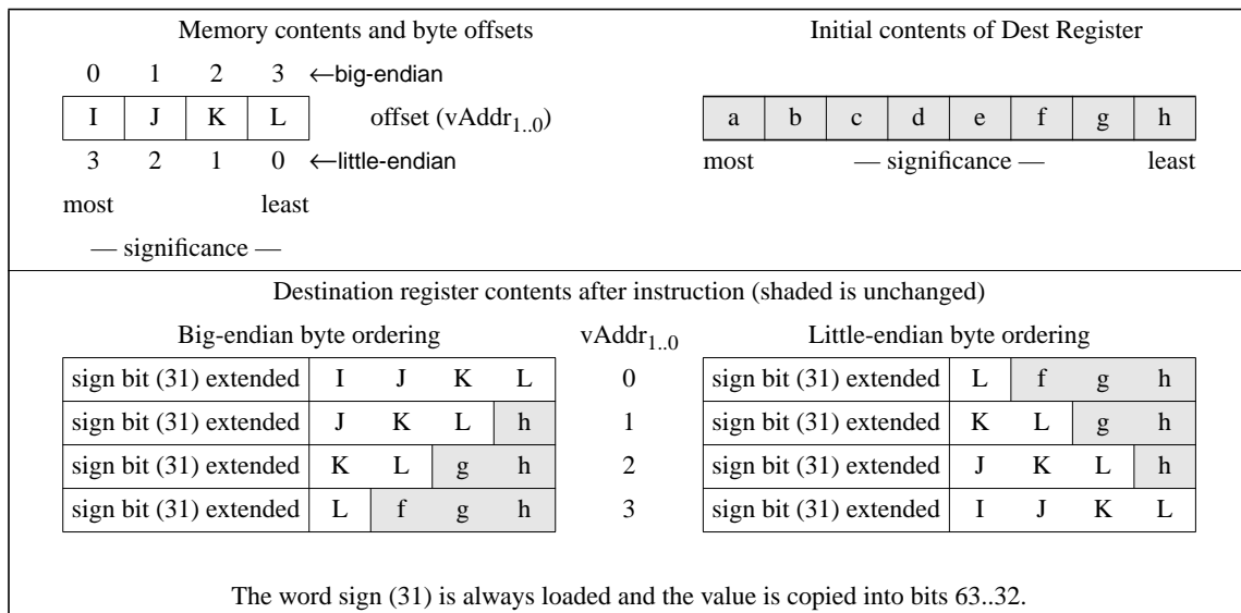
Figure 3-16 Bytes Loaded by LWL Instruction
